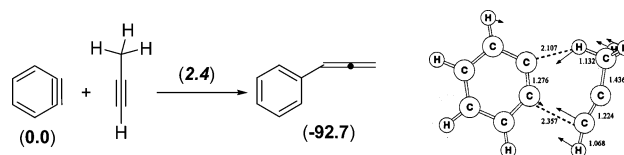
Figure 1. Free energies (kcal/mol) and optimized geometry of the transition state for the reaction of benzyne and propyne. Activation barrier is in italics, and bond lengths are in angstroms.
